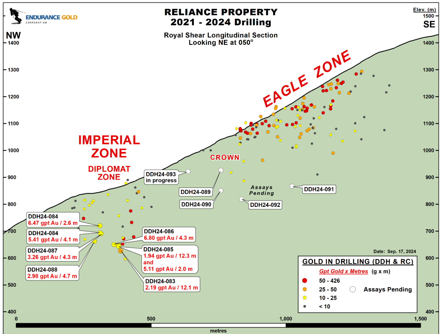
Figure 1: Reliance - Royal Shear Longitudinal Section – 2024 Update & Active Drilling Areas
